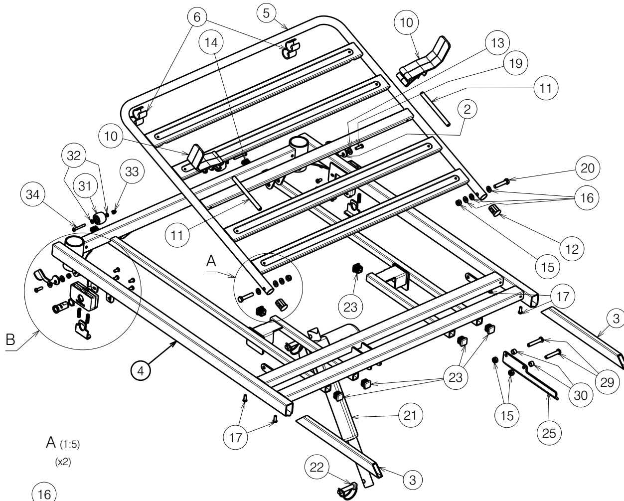
Mattress holder - way of assembly
